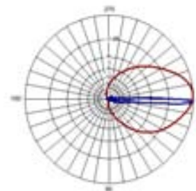
UMTS 2 DEGREE DOWN TILT
