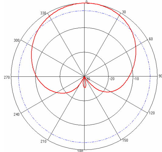
Horizontal Pattern
