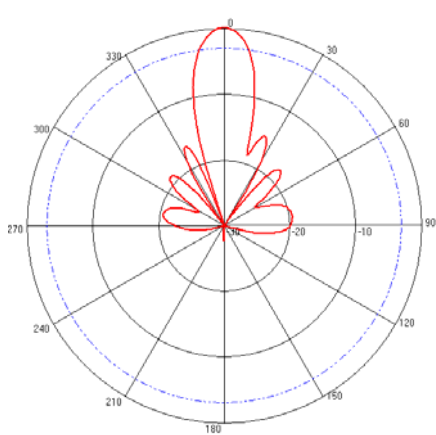
Vertical Pattern
