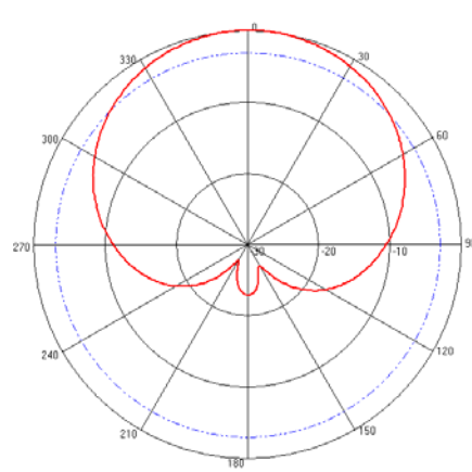
Horizontal Pattern
